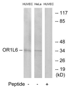
Western blot analysis of extracts from HUVEC cells and HeLa cells, using OR1L6 antibody.
