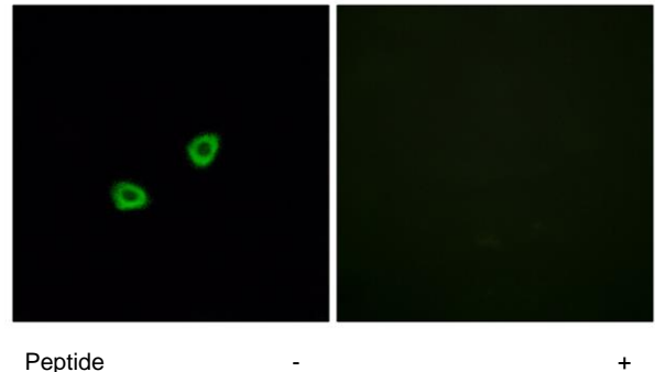
Immunofluorescence analysis of HUVEC cells, using OR1L6 antibody.
