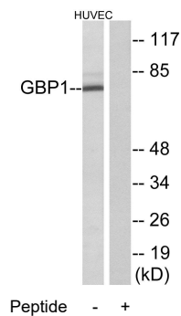
Western blot analysis of extracts from HUVEC cells, using GBP1 antibody.
