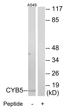
Western blot analysis of extracts from A549 cells, using CYB5 antibody.
